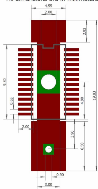
TSSOP-28 LAND PATTERN All dimensions are in millimeters
