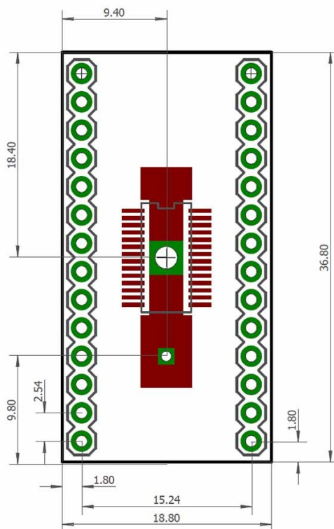
TSSOP-28 BOARD SIZE All dimensions are in millimeters
